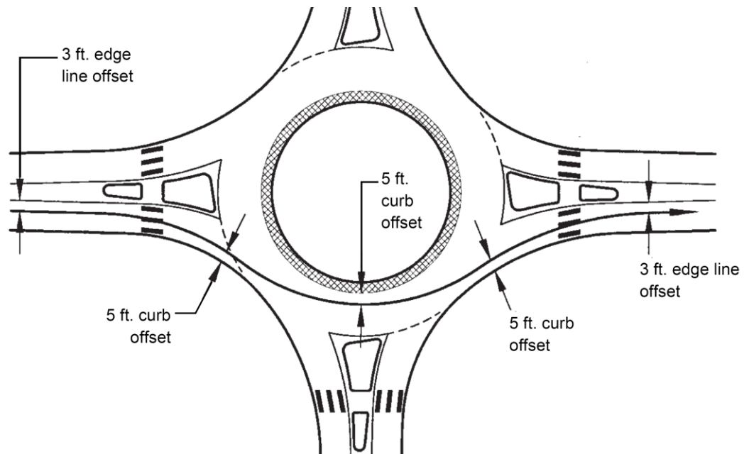
Figure 2-29 Fastest Path for Through Movement at Single Lane Roundabout
