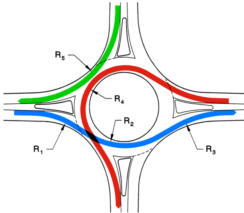
Figure 2-30 Critical Path Radii at a Roundabout
