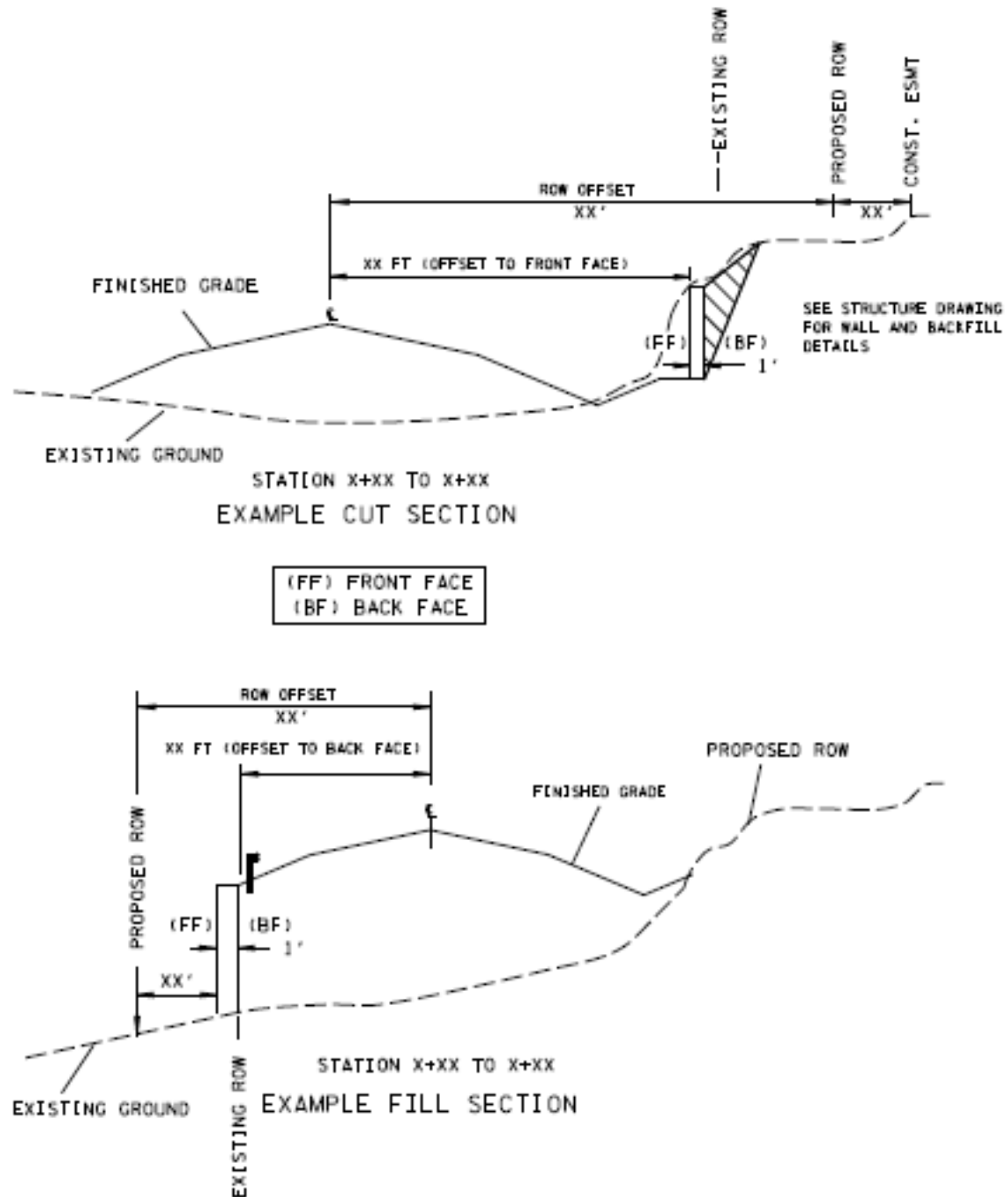
Figure 2-21A Example of Retaining Wall Typical Sections for Cut or Fill Sections
