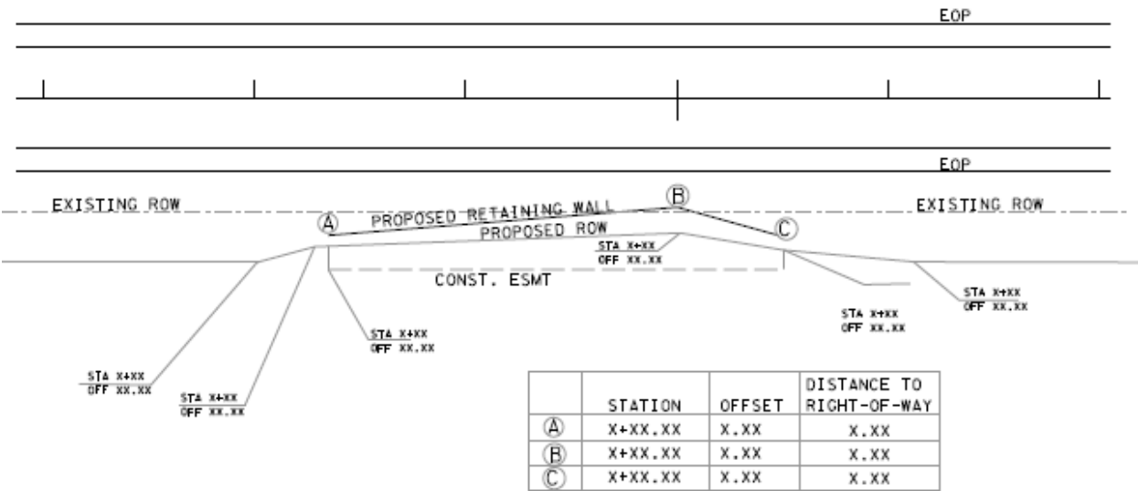
RETAINING WALL LAYOUT DETAILS
