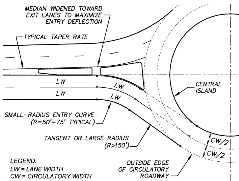
Figure 2-33 Good Path Alignment into Multi-Lane Roundabout Reference: FHWA, Roundabouts Technical Summary (FHWA-SA-10-006)
