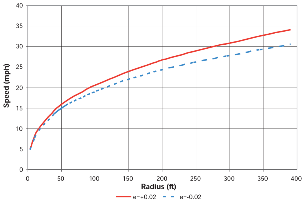
Figure 2-31 Speed-Radius Relationship
